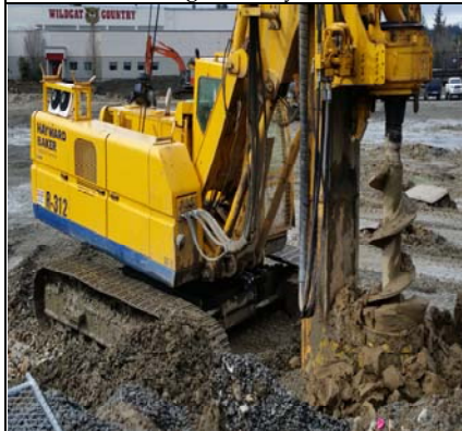
Close Up Of Pilot Hole Drilling
